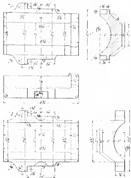
Figs. 5394-5398. BEARING.
